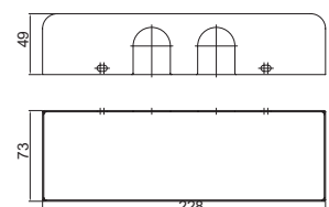
Metal cover
