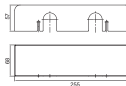
Metal cover
